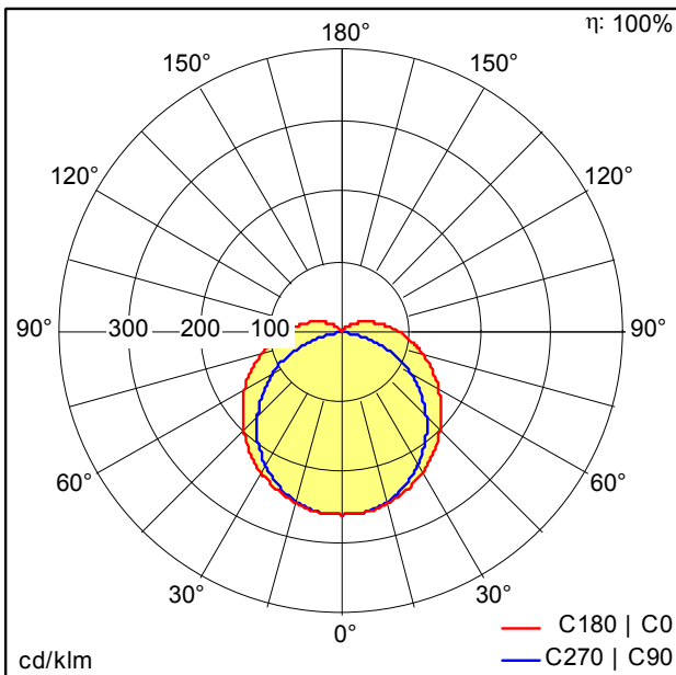
TE_EMMA_LED_1500_6000_840.idt
